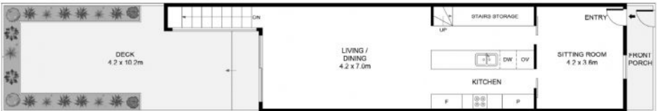
GROUND LEVEL
