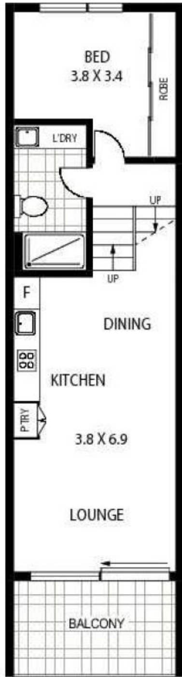
THIRD FLOOR
