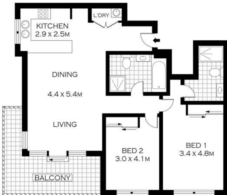
FIRST FLOOR
