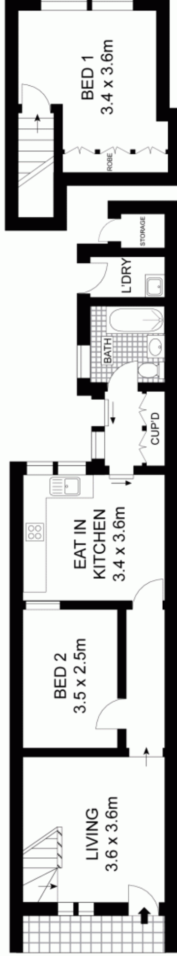
GROUND FLOOR
