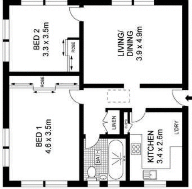
TOP FLOOR
