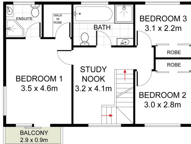
LEVEL ONE
