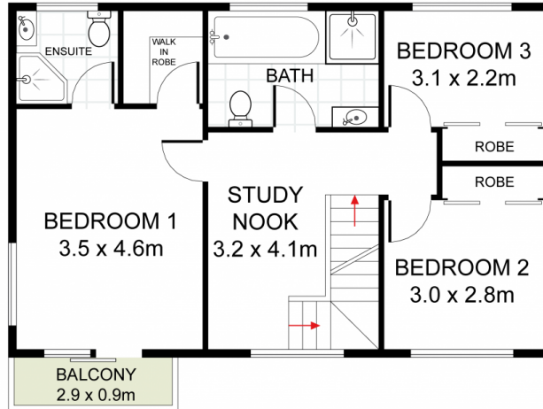
LEVEL ONE
